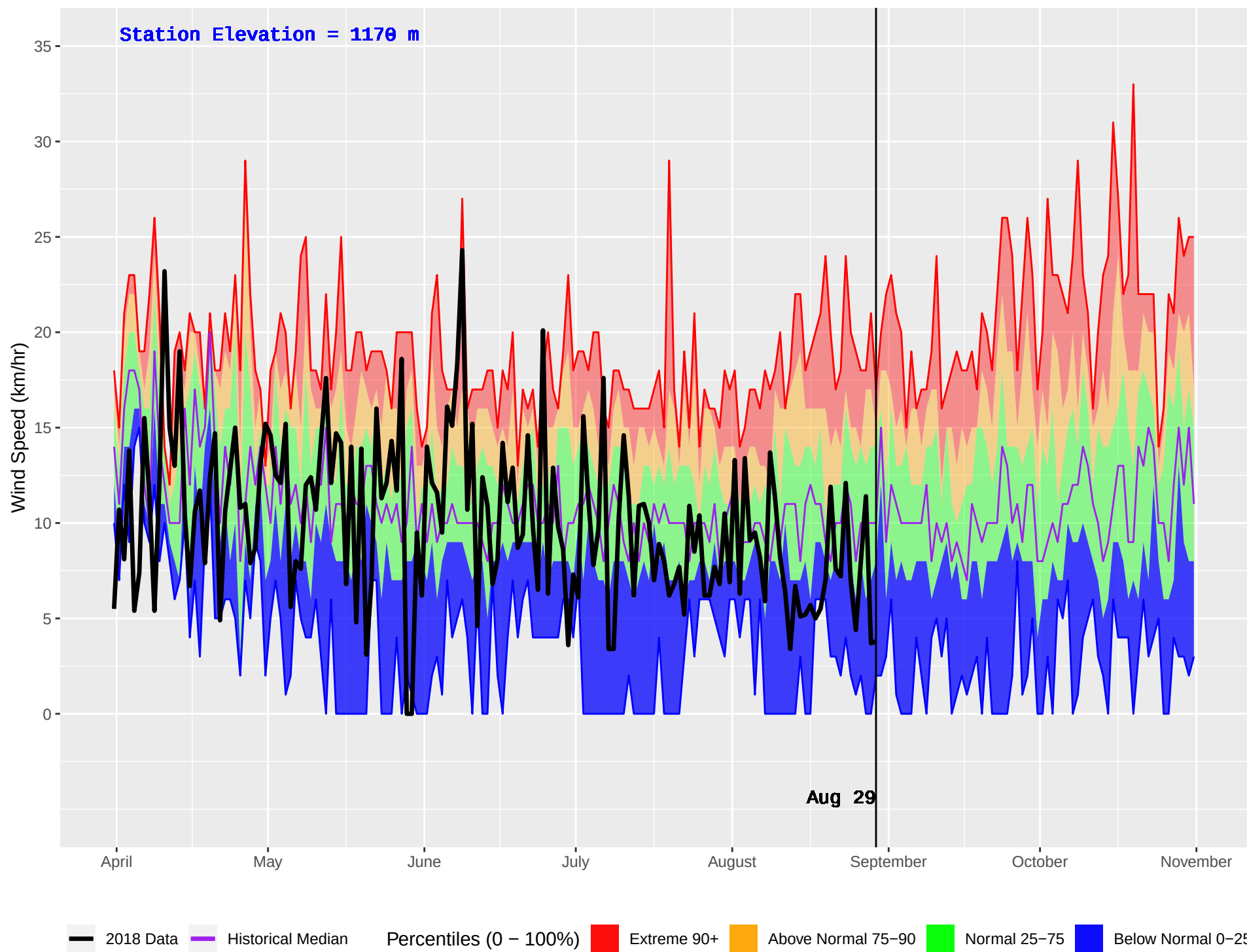
YOUNG LAKE (235) : Historical (2001–2016) and Current (2018) Daily Wind Speed
