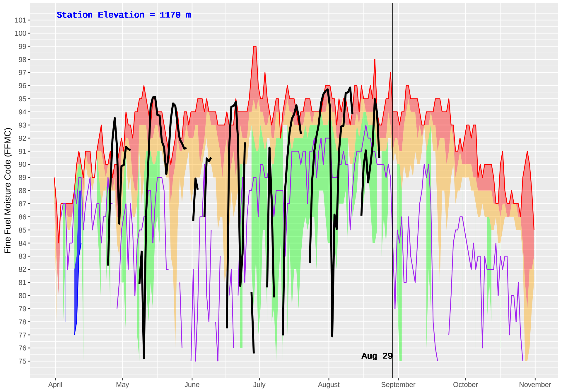
YOUNG LAKE (235) : Historical (2001–2016) and Current (2018) Daily Fine Fuel Moisture Code (FFMC)
